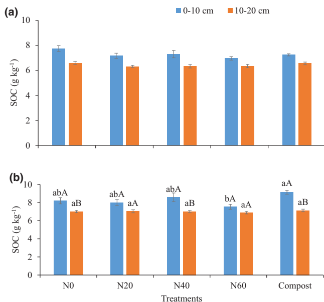
FIGURE 2 Soil organic C under different treatments in 0- to 10- and 10- to 20-cm depths of soil in 2018 (a) and 2019 (b). The N fertilizer rates under N0, N20, N40, and N60 were 0, 22.4, 44.8, and 67.3 kg ha -1 (0, 20, 40, and 60 lb/acre), respectively. Different lowercase letters indicate a significant difference between treatments within a depth, and different uppercase letters indicate a significant difference between depths within a treatment ( p = 0.07 )
