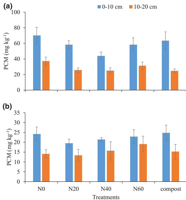
FIGURE 1 Potential carbon mineralization (PCM) under different treatments in 0- to 10- and 10- to 20-cm depths of soil in 2018 (a) and 2019 (b). The N fertilizer rates under N0, N20, N40 and N60 were 0, 22.4, 44.8, and 67.3 kg ha -1 (0, 20, 40, and 60 lb/acre), respectively
