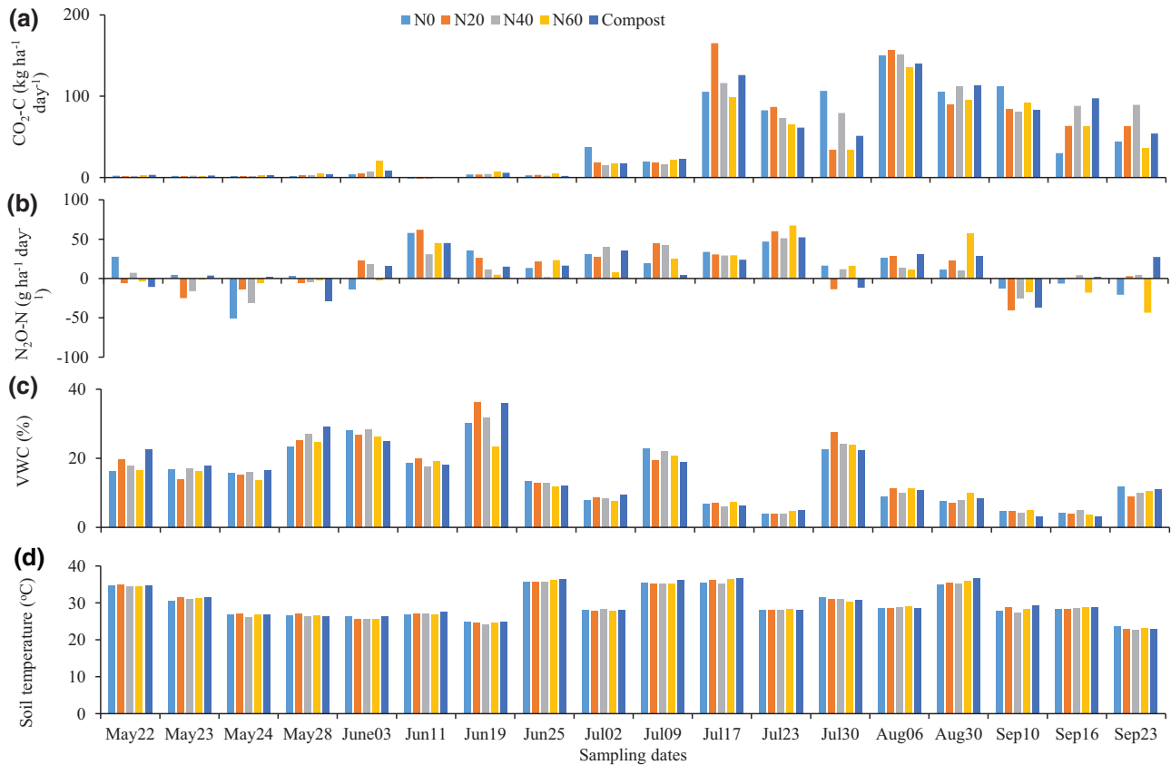
FIGURE 3 Soil (a) CO 2 -C and (b) N 2 O-N emissions, (c) soil water content, and (d) soil temperature in different sampling dates during growing season of 2019. The N fertilizer rates under N0, N20, N40, and N60 were 0, 22.4, 44.8, and 67.3 kg ha -1 (0, 20, 40, and 60 lb/acre), respectively
